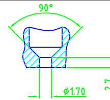
C/Sink Detail
