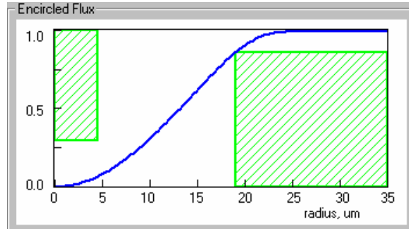
Figure 6. Example of Encircled Flux measurement with IEEE template.
