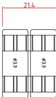
EFA04 71 P03 Ø3.9 COUPLER CLIP
