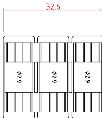
EFA04 71 P01 Ø2.9 COUPLER CLIP
