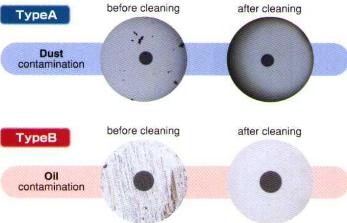
Ferrule end-faces before/after use of the CLETOP series
